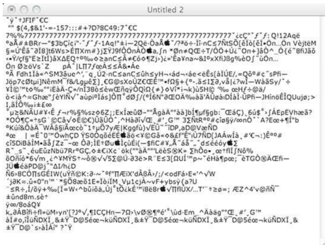
Figure 3.4. Image of a red circle saved as .txt and opened in a text-editor
